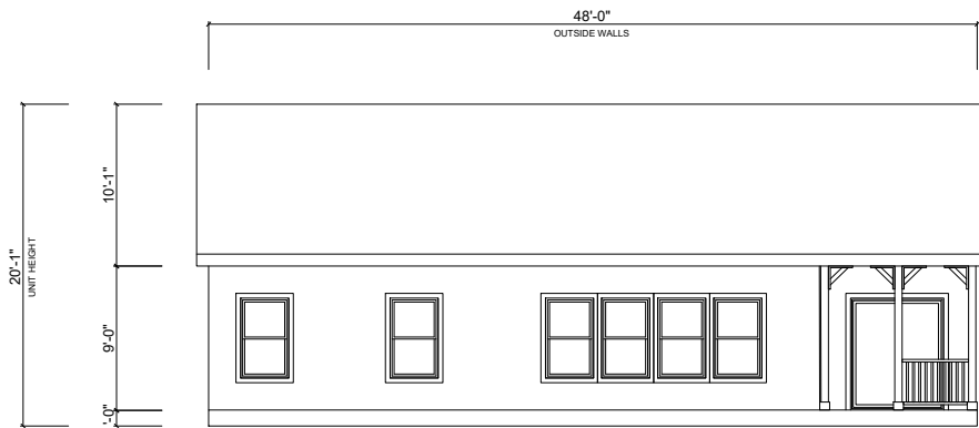
REAR 3
